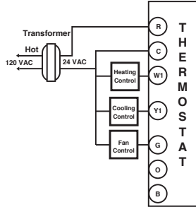
HEAT/COOL 4-WIRE SINGLE TRANSFORMER
