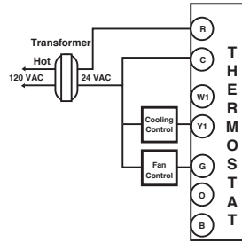
COOL ONLY 3-WIRE SINGLE TRANSFORMER
