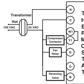
HEAT PUMP WITH HEAT ACTIVE REVERSING VALVE
